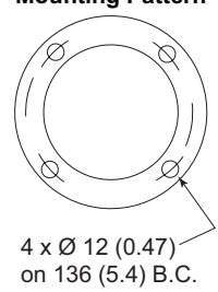
Mounting Pattern
