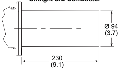
Straight SiC Combustor
