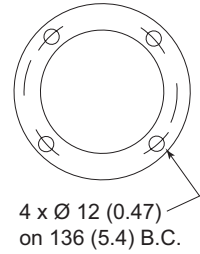
Mounting Pattern
