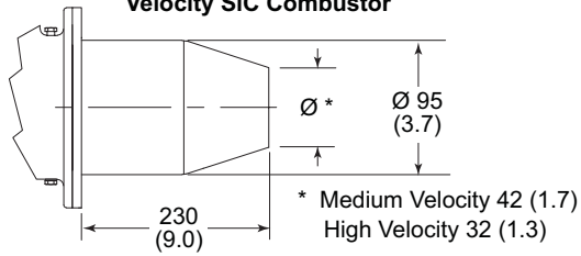
Medium & High Velocity SiC Combustor
