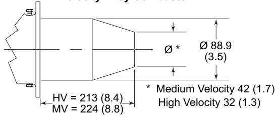
Medium & High Velocity Alloy Combustor
